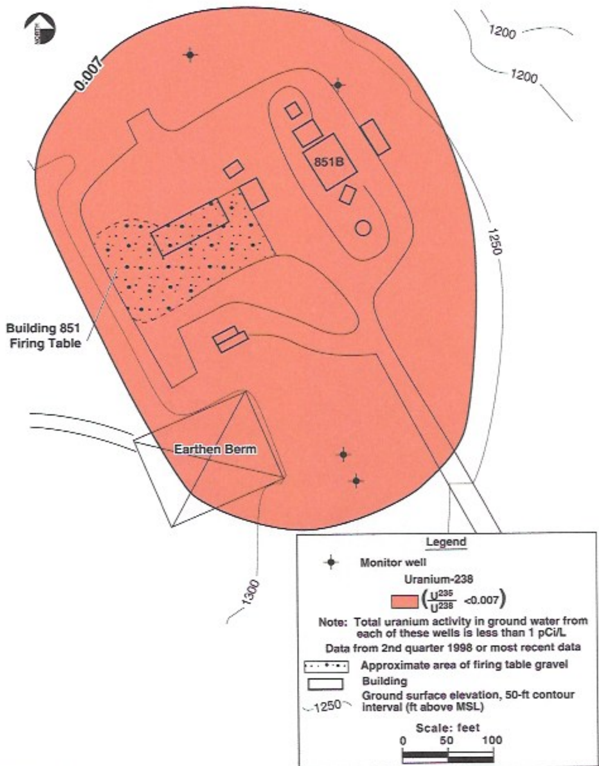
Figure 1-42. Distribution of uranium-238 in ground water in the Building 851 Firing Table area, OU8.
